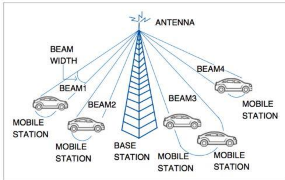
Figure 4 Beam-division multiple access Framework
